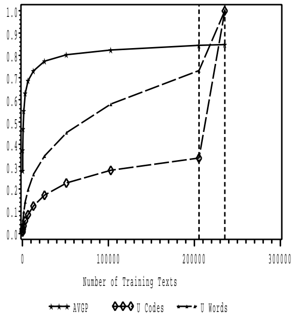
Figure 2: Learning curve of ExpNet using sort-and-split sampling.
